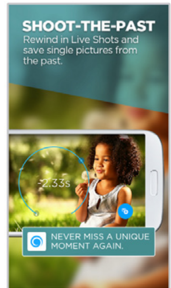
Camera MX
