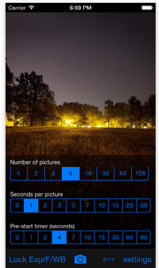
Average CameraPro
