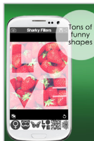
Rookie
