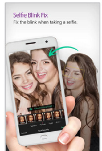
YouCam Perfect
