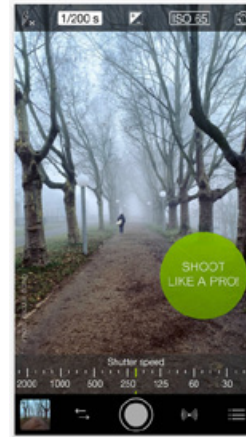
ProCamera
